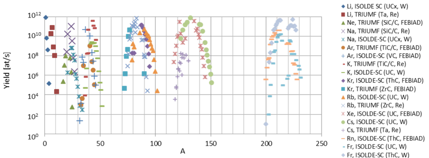
ISOL@MYRRHA yields for alkalis and noble gases from ISOLDE-SC and TRIUMF extrapolations
